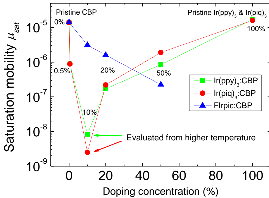
Fig. 5. The saturation hole mobilities of doped CBP films using \text{Ir(ppy)}_3 , \text{Ir(piq)}_3 and Flrpic as dopants. The doping concentration varies from 0% (undoped CBP) to 100% (neat film of dopant). The data for \text{CBP:Ir(ppy)}_3 and \text{CBP:Ir(piq)}_3 were obtained at 390 K.
