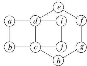
Figure 5.1: A polygonal tree.
