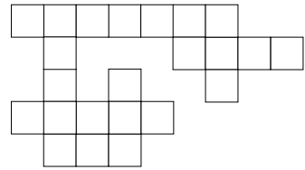
Figure 4.1: A polyomino.
