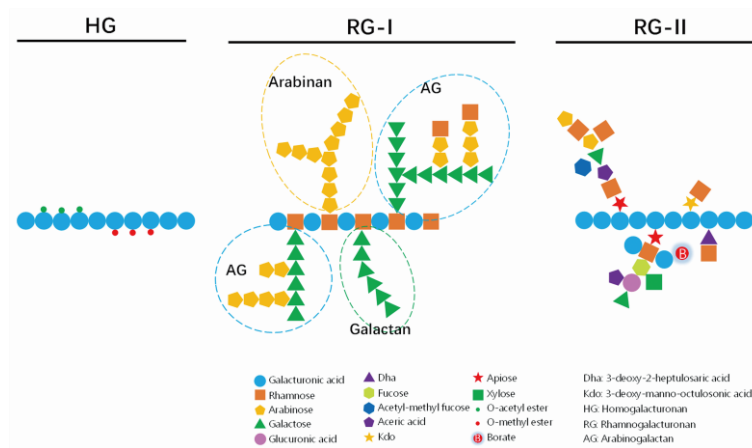
Figure 1. Schematic illustration of representative ginseng pectins.
