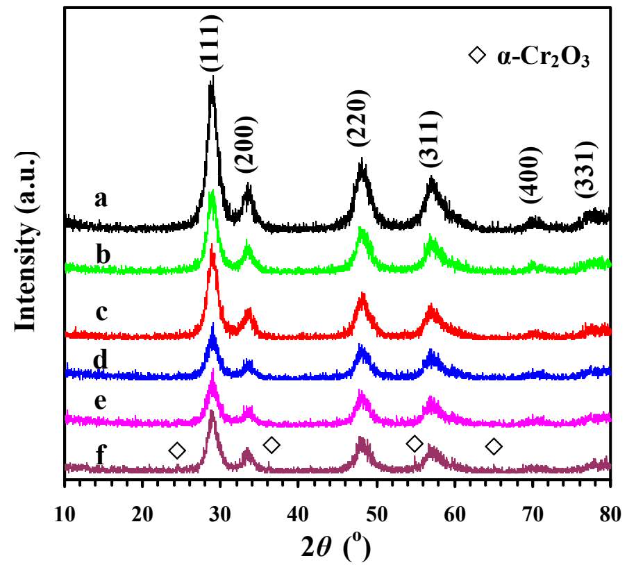
Fig. 1. XRD patterns of y \text{CrO}_x/\text{nano-CZY} samples with y = (a) 0, (b) 2, (c) 4, (d) 6, (e) 8, and (f) 10 wt%.
