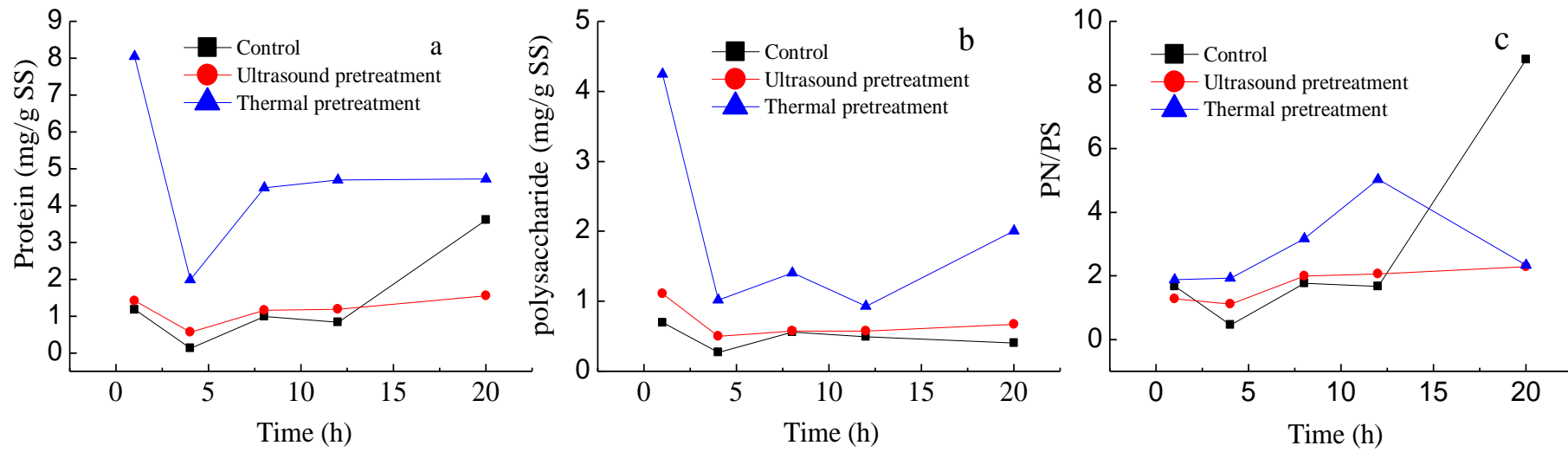
Figure S2: Variation of the content of protein (a), polysaccharide (b) and PN/PS (c) in the LB-EPS during sludge anaerobic digestion process (PN/PS: protein/ polysaccharide)
