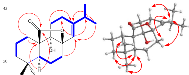
Fig. 3 Key COSY (—in blue), HMBC (→in red) and ROESY (↔in red) correlations for 2 .
