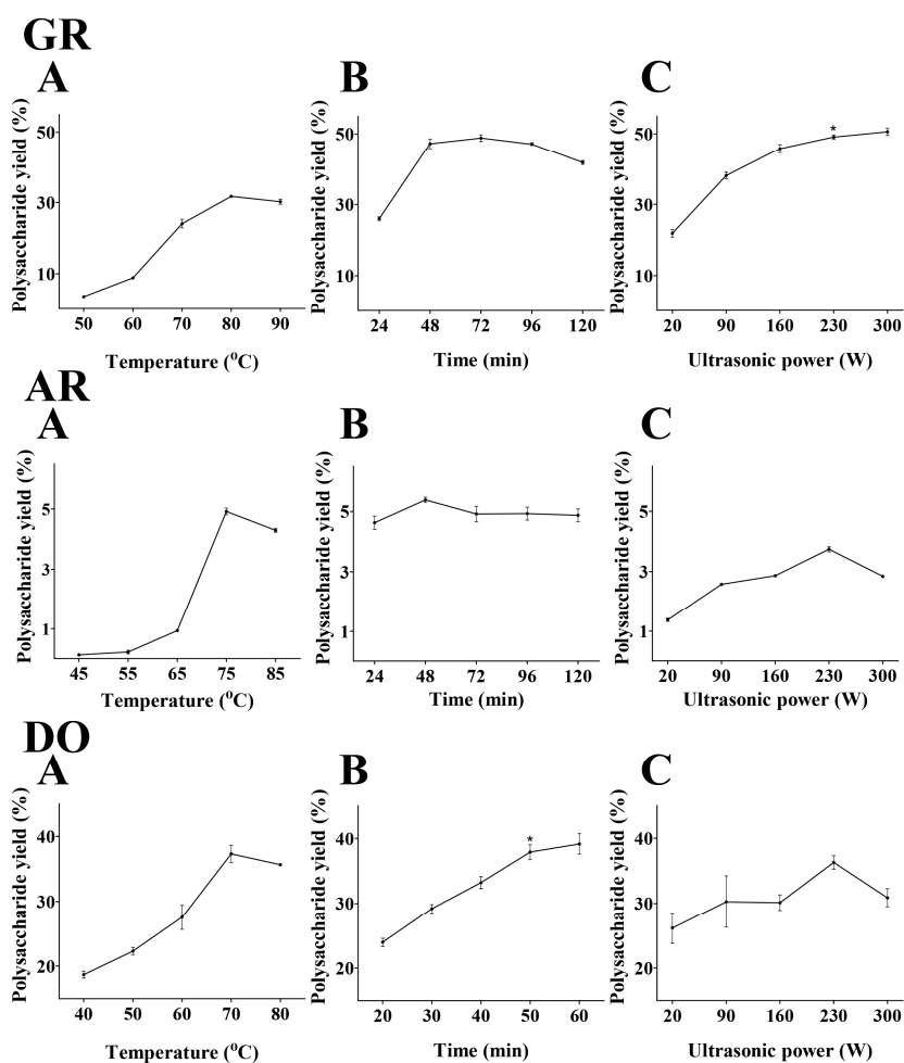
Figure S1. Effect of different temperature (A); extraction time (B) and ultrasonic power (C) on the polysaccharide yield in the herbal samples by single-factor test.* p < 0.05 , compared with the previous one.
