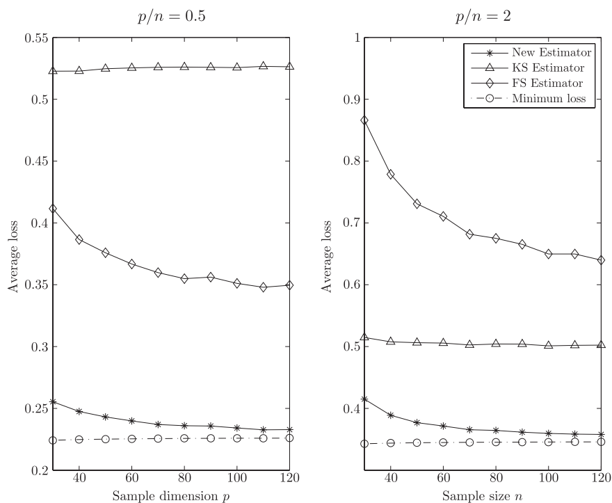
Figure 1. Average losses of the new estimator and the competitors for different combinations of p and n , where the data are Gaussian distributed and the covariance matrix is generated using Model 2. The minimum losses L_0 are reported for comparison.
