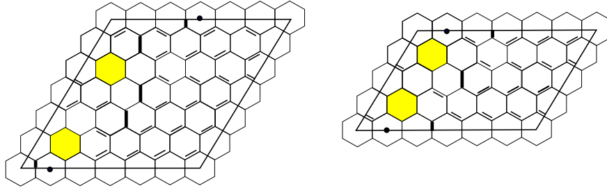
Figure 5: Illustration for Case 1 in the proof of Lemma 3.3.
