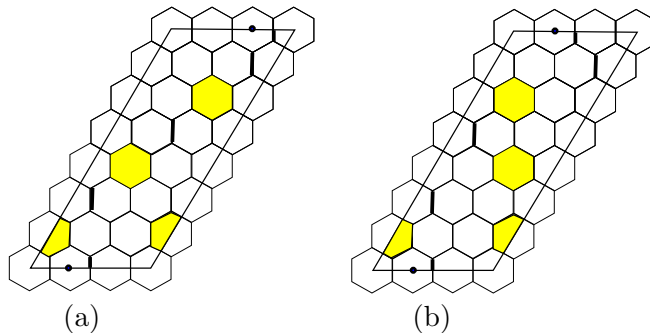
Figure 10: An ideal configuration of H(3, 7, t) for (a) y_2 = 3, y_3 = 5 and t = 1 , (b) y_2 = 5, y_3 = 3 and t = 0 .
