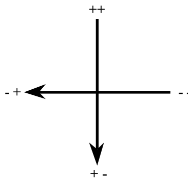
Figure 3: The Cross as a 2LAR Map
